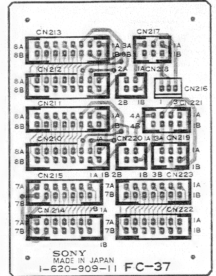
1-620-909-11 COMPONENT SIDE 1-620-909-11 SOLDER SIDE
